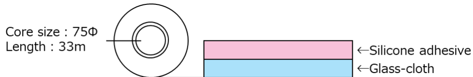
Fig.1 Structure
